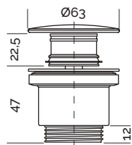
Válvula clic-clac Akron (mm)
