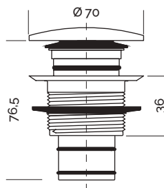
Válvula clic-clac Akron (mm)
