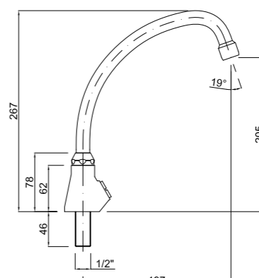
Caño tubo cisne 18 mm, 1/2" giratorio 1/2" tabletop spout, "swan" model Bec 1/2" 18mm
