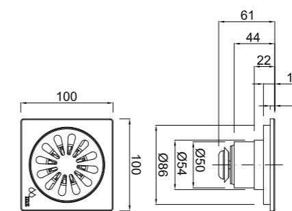
Sumidero inspeccionable 10 x 10 cm Ø 50 mm, con válvula antiretorno Self-closed floor drain, 10 x 10 cm, untireturn valve, Ø 50 mm Vidage Douche Encastré Reviewable
